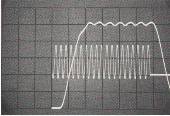
Fig. 10. Oscilloscope showing burst-frequency measurement to 4% accuracy. Number of cycles needed is 6.3, one more than that shown in Fig. 9 because of one-cycle delay in divide-by-two multivibrator.
