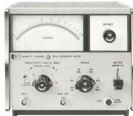
Fig. 1. New -hp- Model 5210A Frequency Meter and FM Discriminator directly measures frequencies between 3 Hz and 10 MHz. Special log-linear meter scale can be read accurately within \pm 1\% of reading. Discriminator output is useful for measurements of instantaneous frequencies of FM signals, measurements that are impossible for most other frequency measuring devices.
